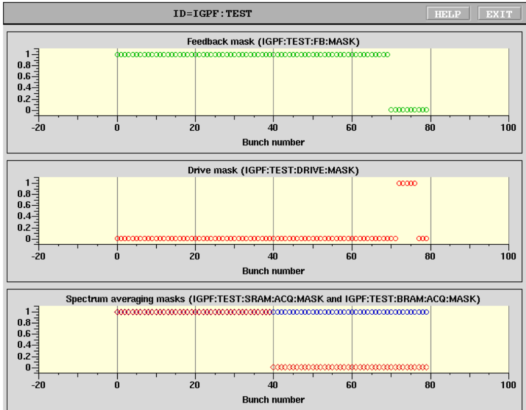
Figure 18: Bunch enable masks panel
