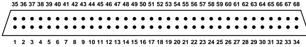
Figure 27: Pin numbering for general-purpose digital I/O connector
