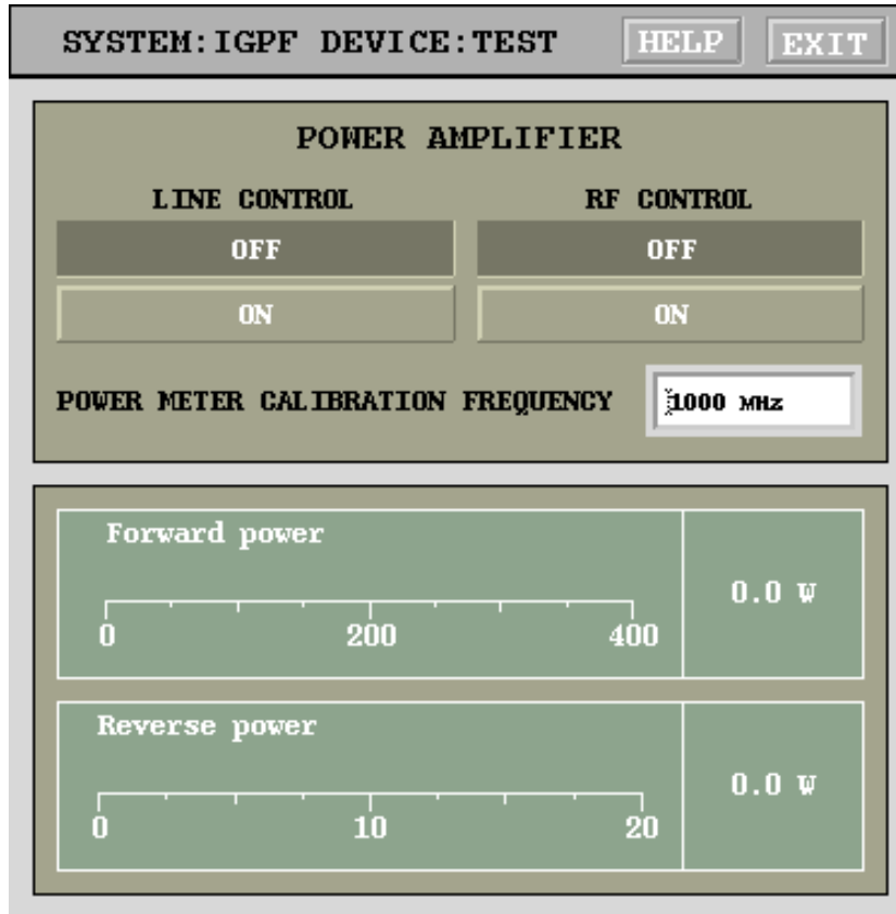
Figure 24: Power amplifier control and monitoring panel
