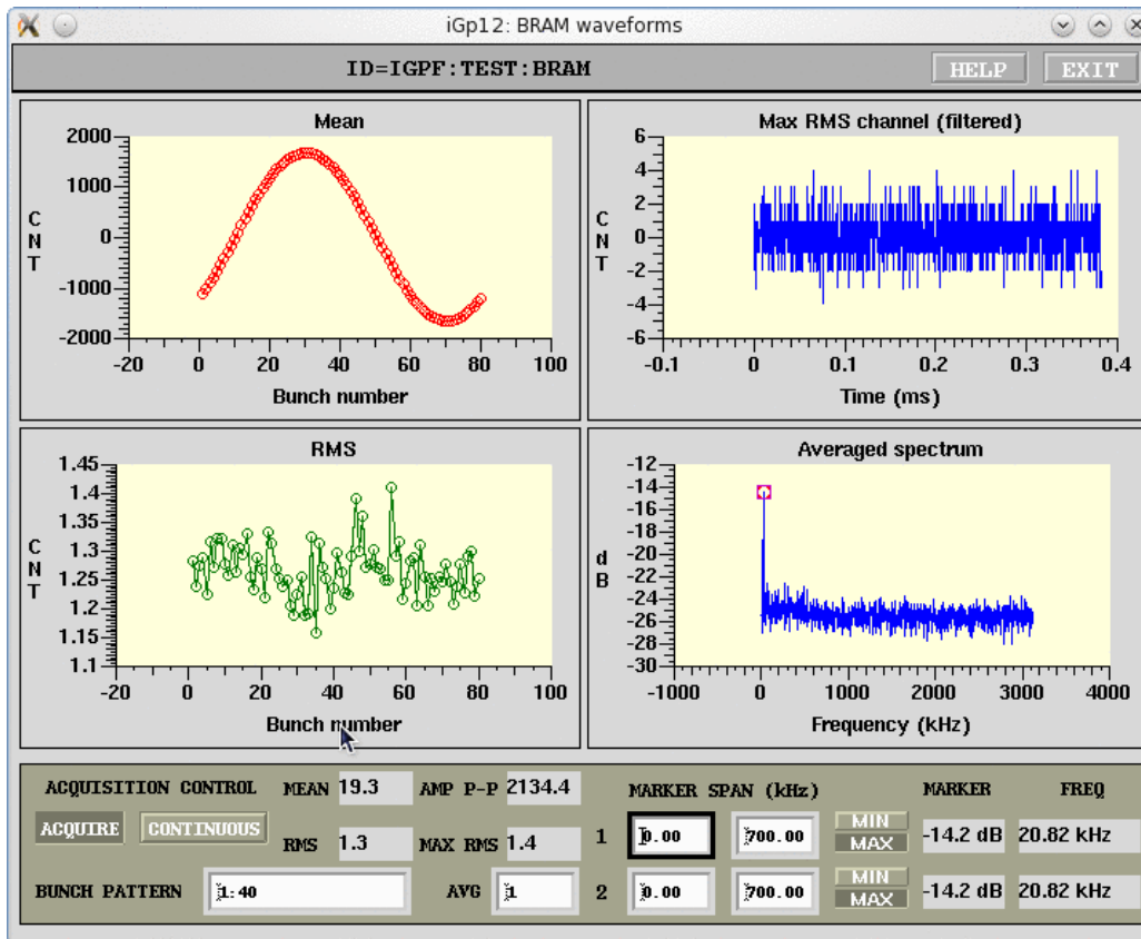
Figure 15: Waveforms panel
