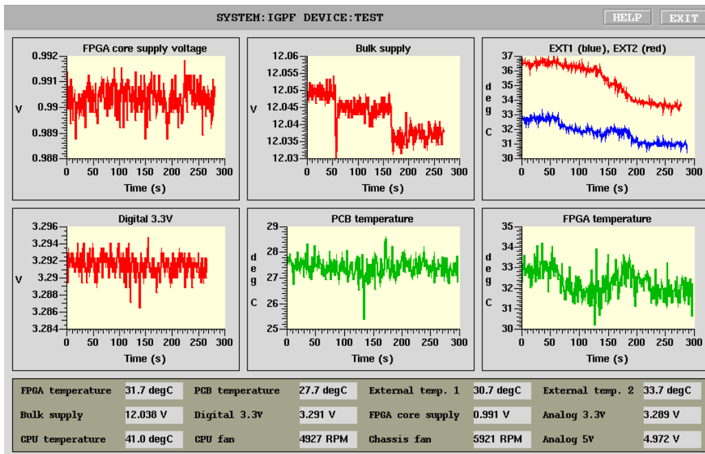
Figure 16: Environmental monitoring panel
