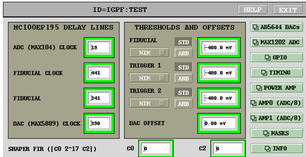
Figure 17: Device controls panel
