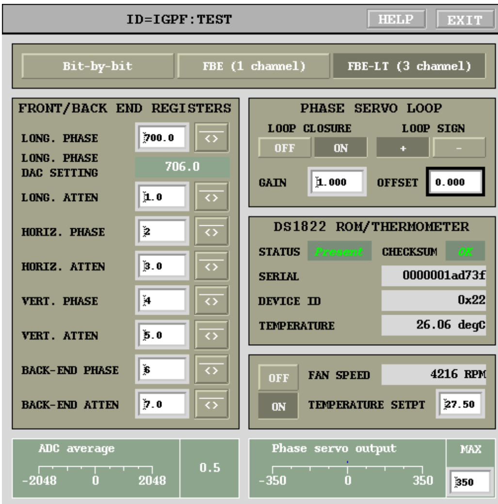
Figure 23: General-purpose I/O panel: FBE-LT driver
