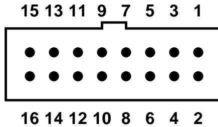
Figure 26: Pin numbering for 16-pin header-type front-panel connectors
