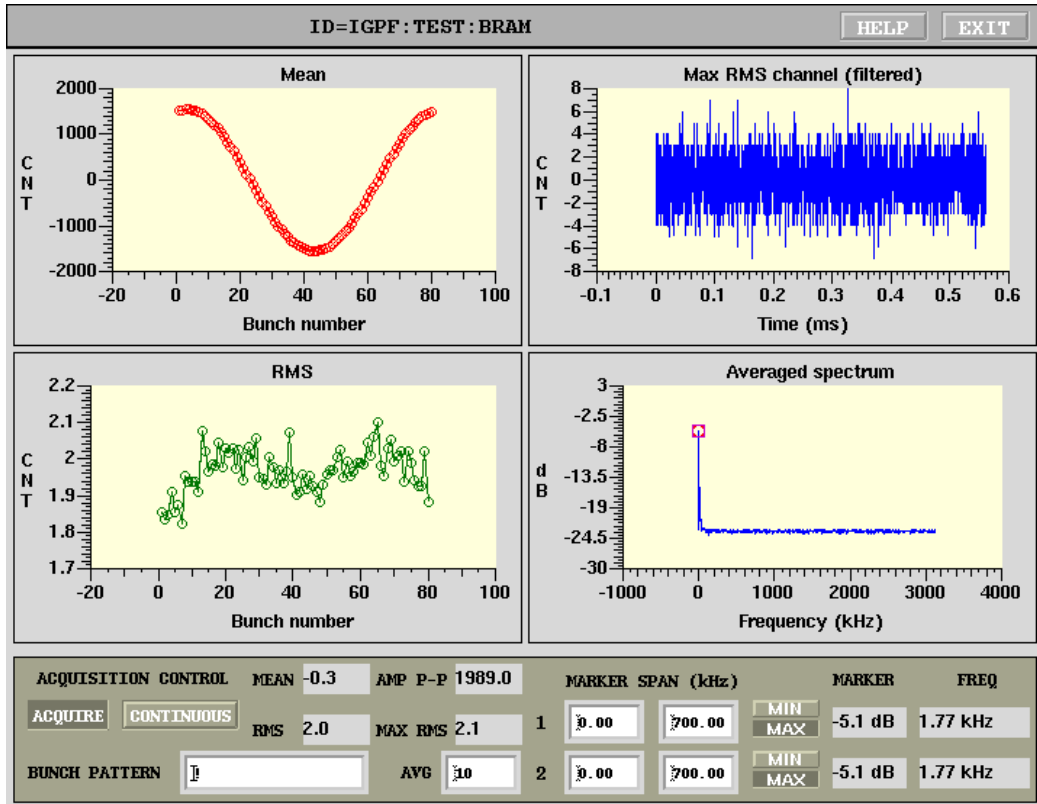
Figure 18: Waveforms panel
