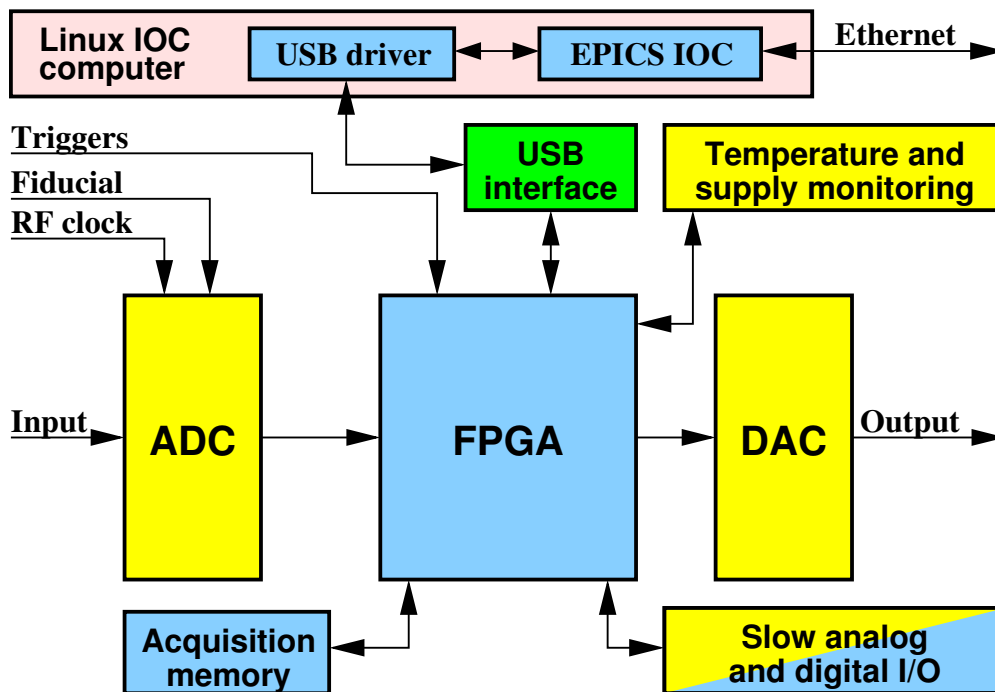
Figure 1: iGp12-328F block diagram
