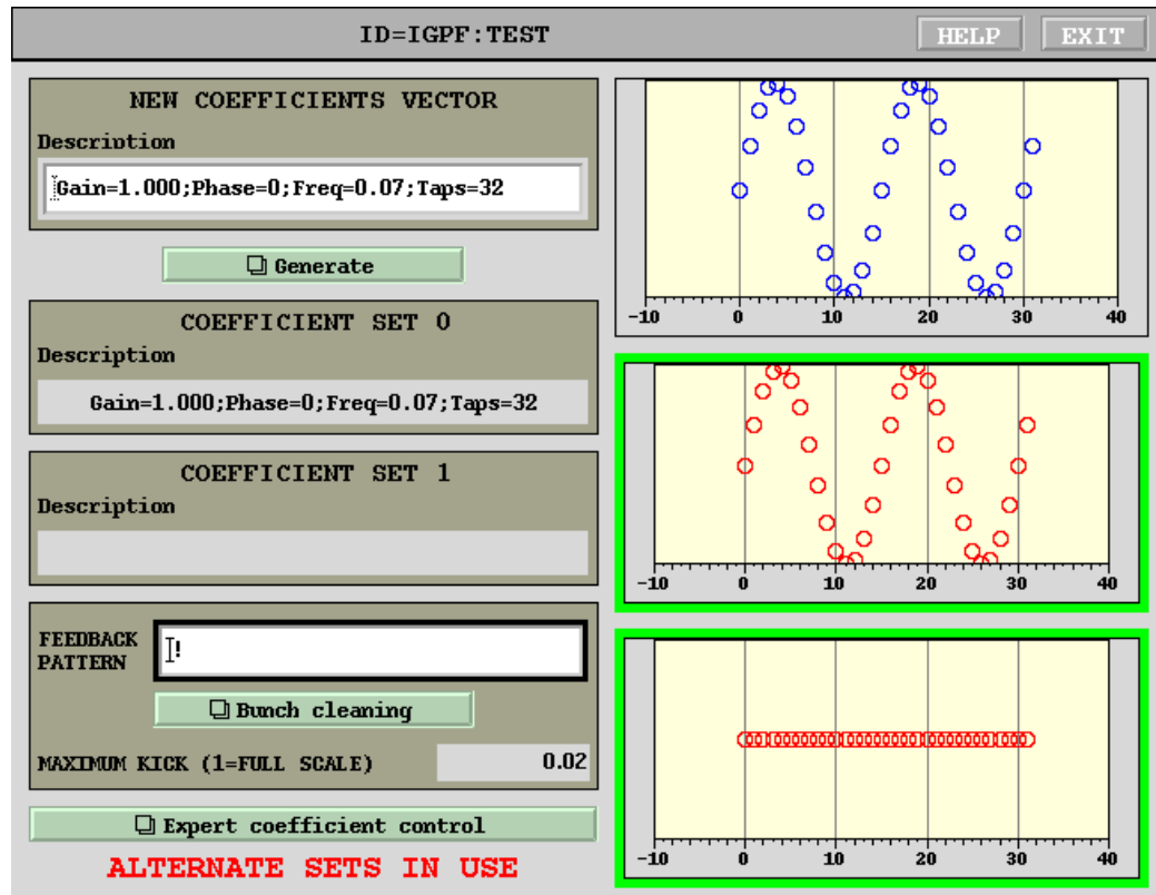
Figure 10: Coefficients panel
