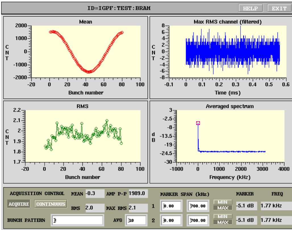
Figure 18: Waveforms panel
