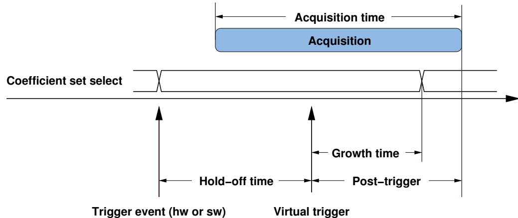
Figure 6: Multi-bunch acquisition process: timing relationships.
