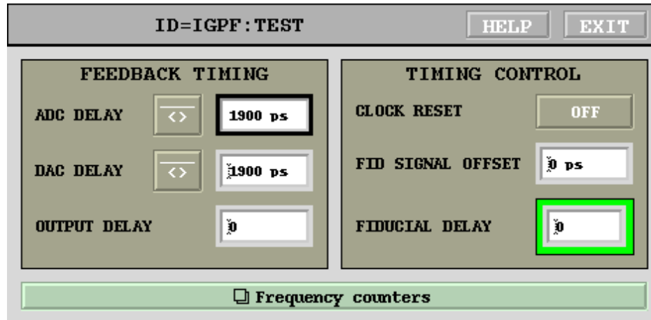
Figure 14: Timing panel
