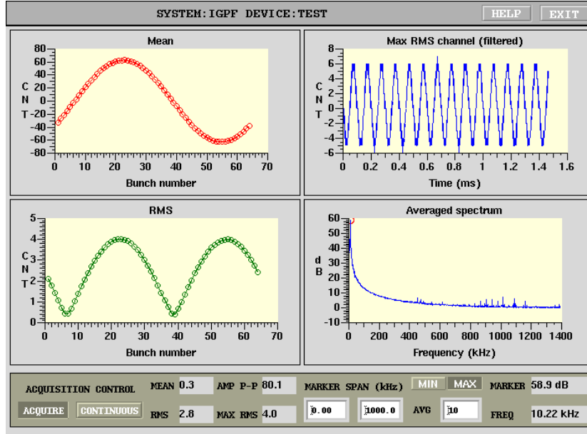
Figure 11: Waveforms panel
