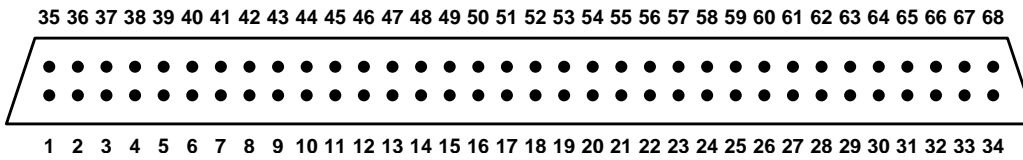
Figure 19: Pin numbering for general-purpose digital I/O connector
